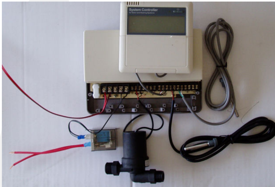
Fig 4. Wiring example.
