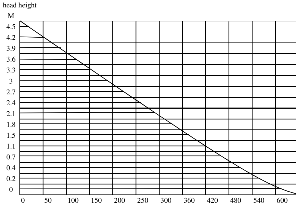
Figure 2. Static head in meters versus flow rate in L/h.
